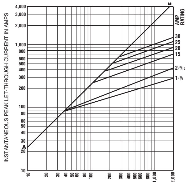
PROSPECTIVE SHORT-CIRCUIT CURRENT—SYMMETRICAL RMS AMPS
