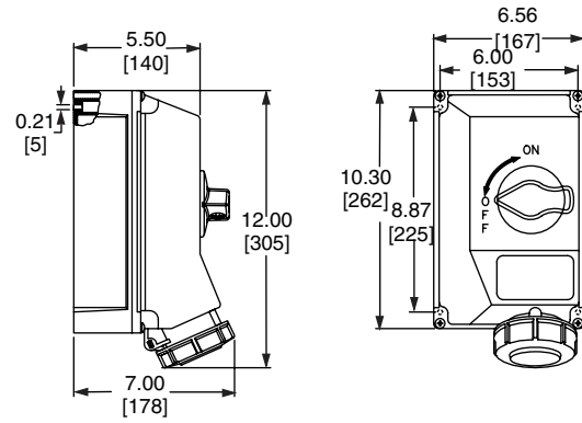
30 A Non-Fusible
