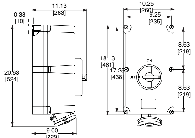
100 A Non-Fusible
