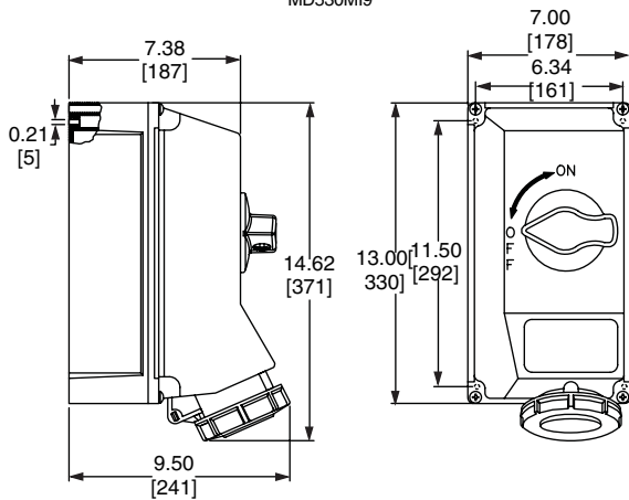
60 A Non-Fusible
