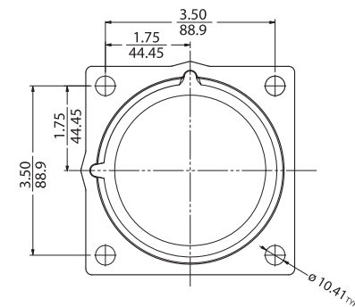
Panel Receptacle Flange
