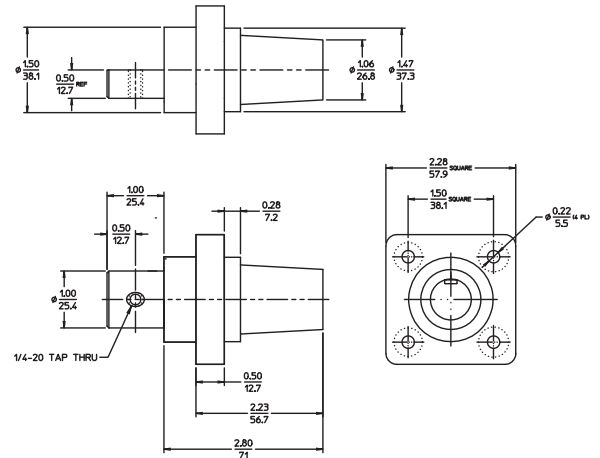
16R20 Female Panel Receptacle Bus Bar Version
