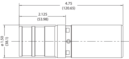
Female Contact
