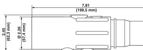
Ball Nose In-line Latching Male Connectors - Crimped
