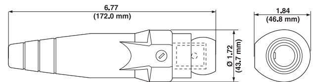
Female Detachable Plug – Single Set Screw
