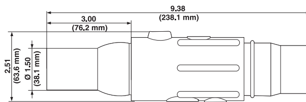
Female Detachable Plug - Double Set Screw
