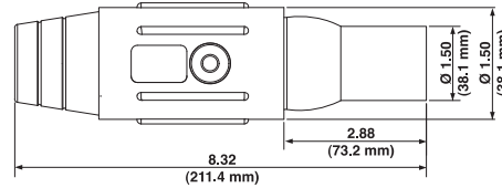
Ball Nose In-line Latching Female Connectors S-Series
