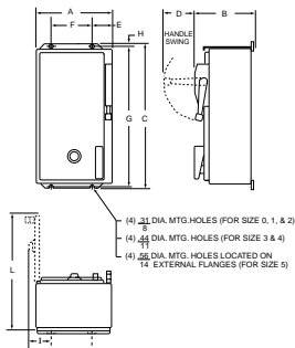
Figure 4 NEMA Type 12 Enclosure
