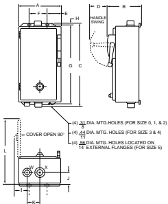
Figure 3 NEMA Type 4 Enclosure
