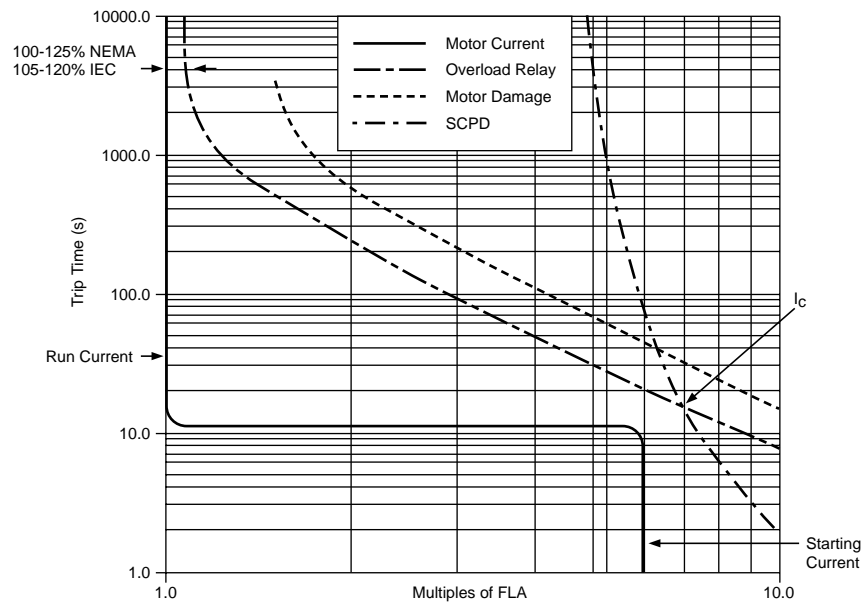
Figure 2 Typical Coordination Curves
