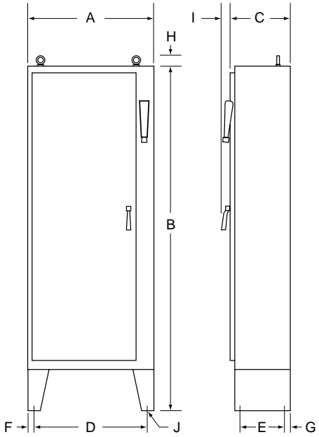
Enclosure Style 5
